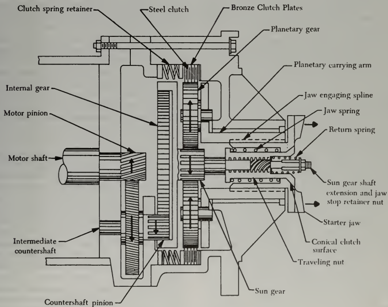
FIGURE 5-8. Starter gear section.
